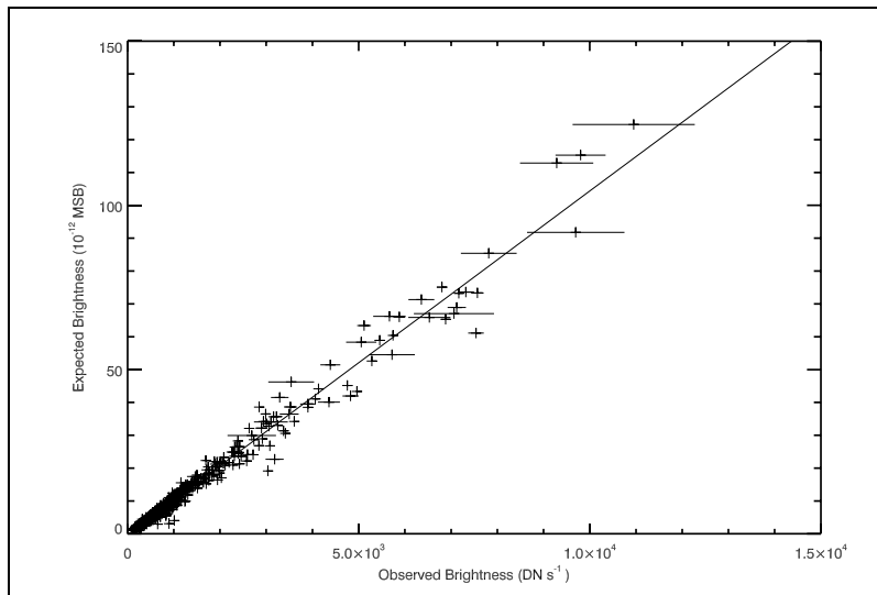
Figure 3 The measured flux from the 2011 observations against the expected stellar brightness in COR2-A. The slope of the fit line gives the photometric calibration factor in units of (MSB)/(DN s-1 pixel-1).
