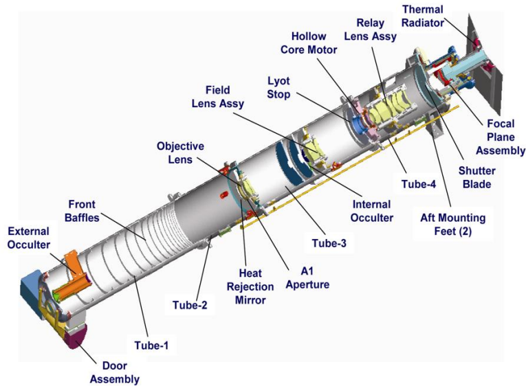
Figure 1 COR2 opto-mechanical layout
