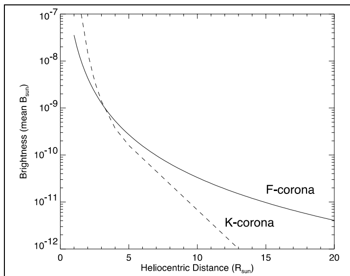
Figure 5 Model equatorial brightness curves for K corona (Saito et al. 1977) and F corona (Koutchmy & Lamy 1985). The F corona dominates the observed signal for heliocentric distances larger than about 4 R_s . From Hayes et al. (2001)
