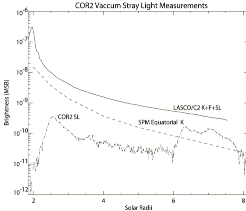
Figure 2. Comparison of the stray light levels in COR2 against the expected F and K coronal levels from LASCO/C2 and the Saito-Poland-Munro (1972) model.
