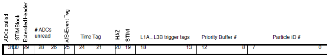
Figure 2.2: Event Record Header, 32 bits.
