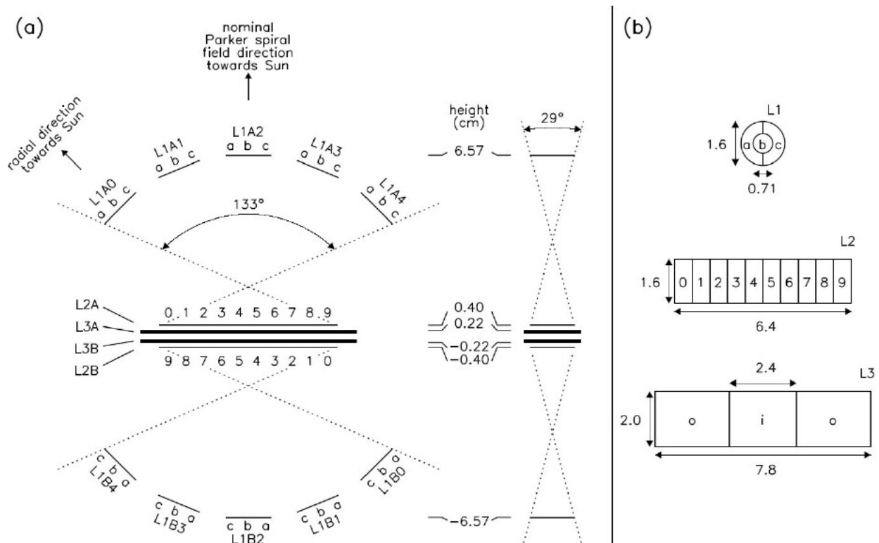
Figure 1: LET Instrument Cross-Section
