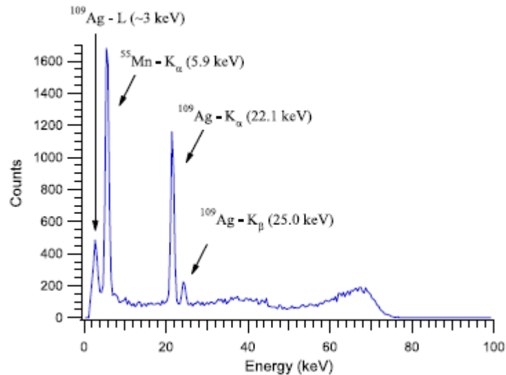
Figure 3: Spectrum obtained by illuminated a STE detector at ambient temperature with a source of one \mu\text{Ci} ^{55}\text{Fe} and a one \mu\text{Ci} ^{109}\text{Cd} simultaneously. The integration time is not sufficient to show the 88 keV gamma emission of the ^{109}\text{Cd} . The broad peaks centered around 68 keV and 40 keV are due to the 84 and 62 keV ^{109}\text{Cd} conversion electrons that have lost energy in the source and detector Windows. A combination of ^{109}\text{Cd} and ^{55}\text{Fe} radioactive source to the inside of the door provides in-orbit calibration of the SSDs when door is closed
