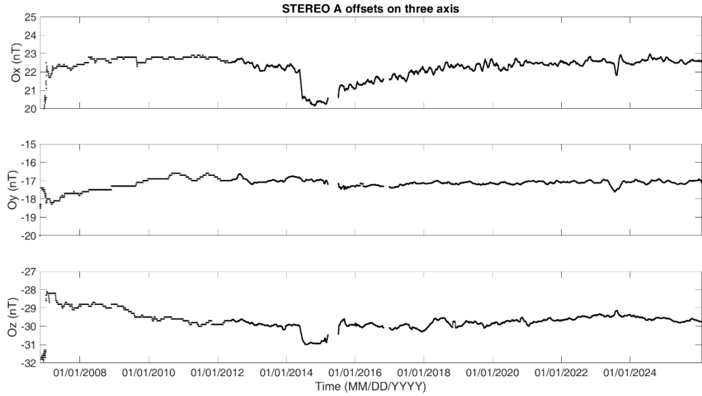
Figure 1. The offsets on three sensor axes of STEREO A.
