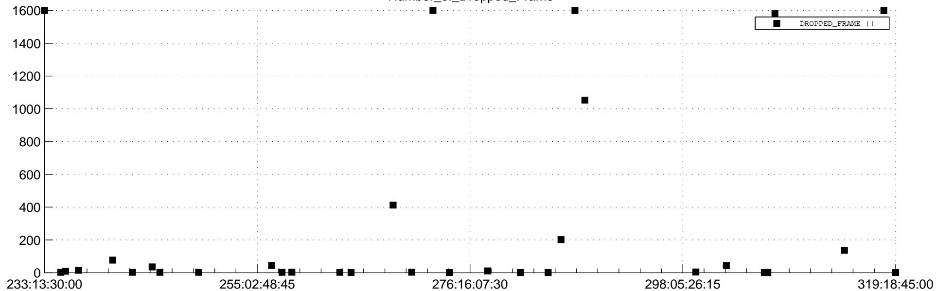
Number_of_Dropped_Frame
