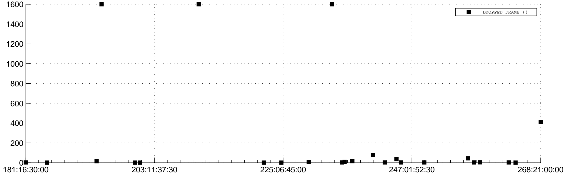
Number_of_Dropped_Frame
