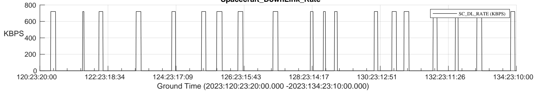
Spacecraft_DownLink_Rate
