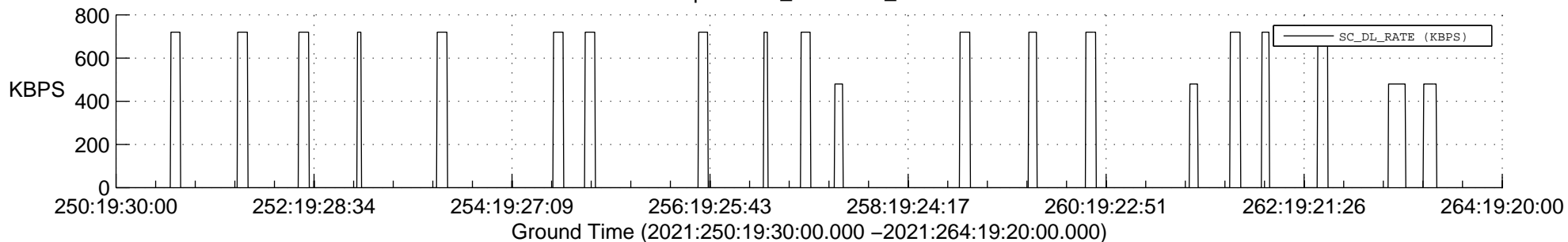
Spacecraft_DownLink_Rate
