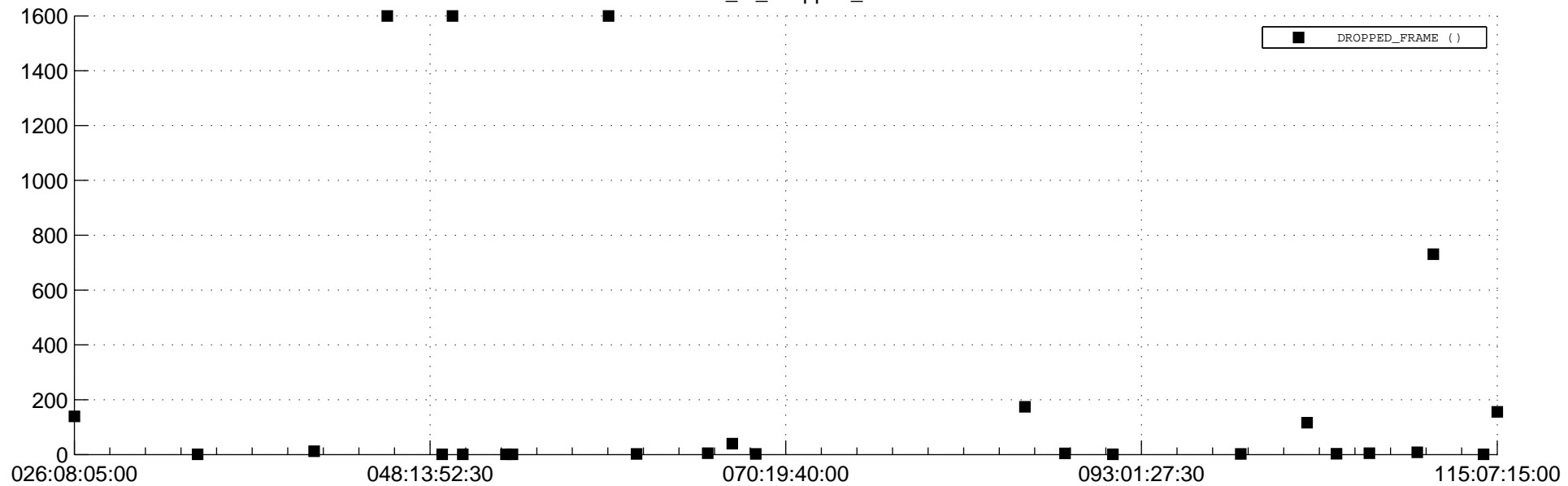
Number_of_Dropped_Frame
