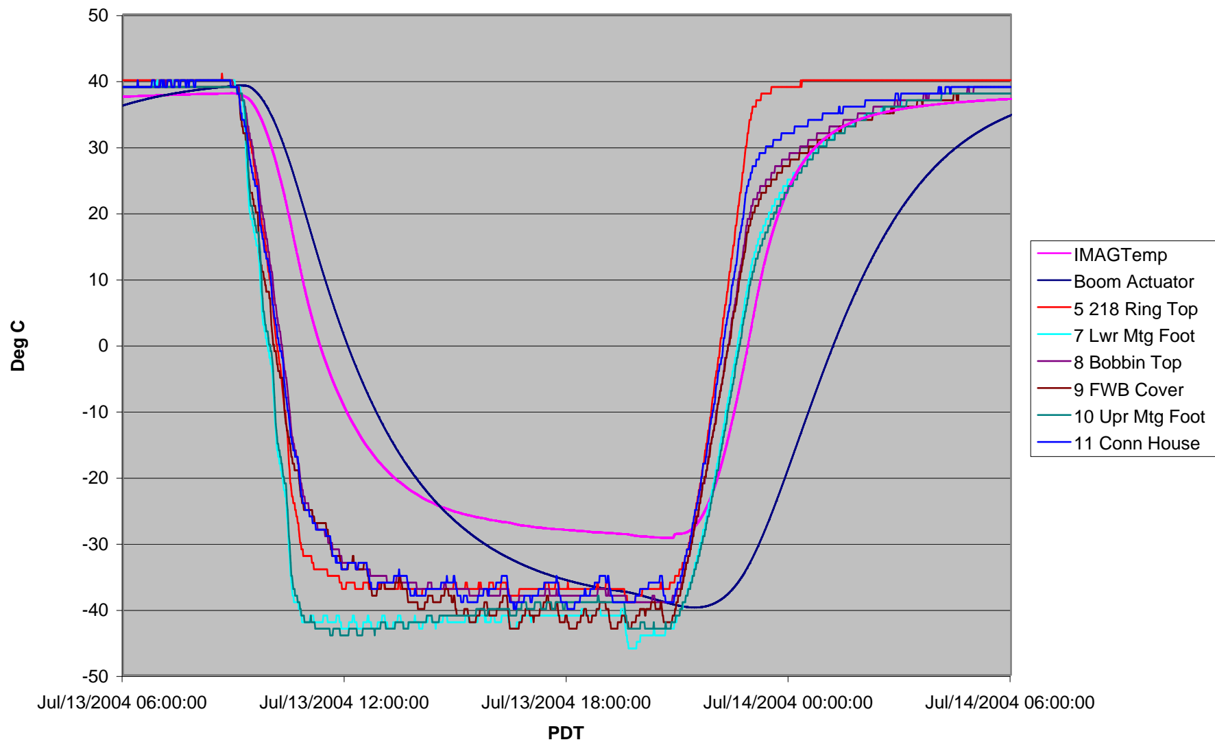
FM1 Boom Thermal Vac, Cycle #6
