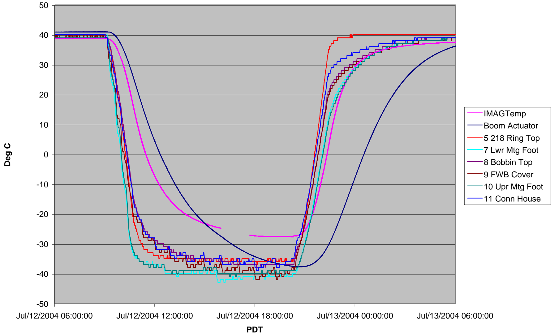
FM1 Boom Thermal Vac, Cycle #5
