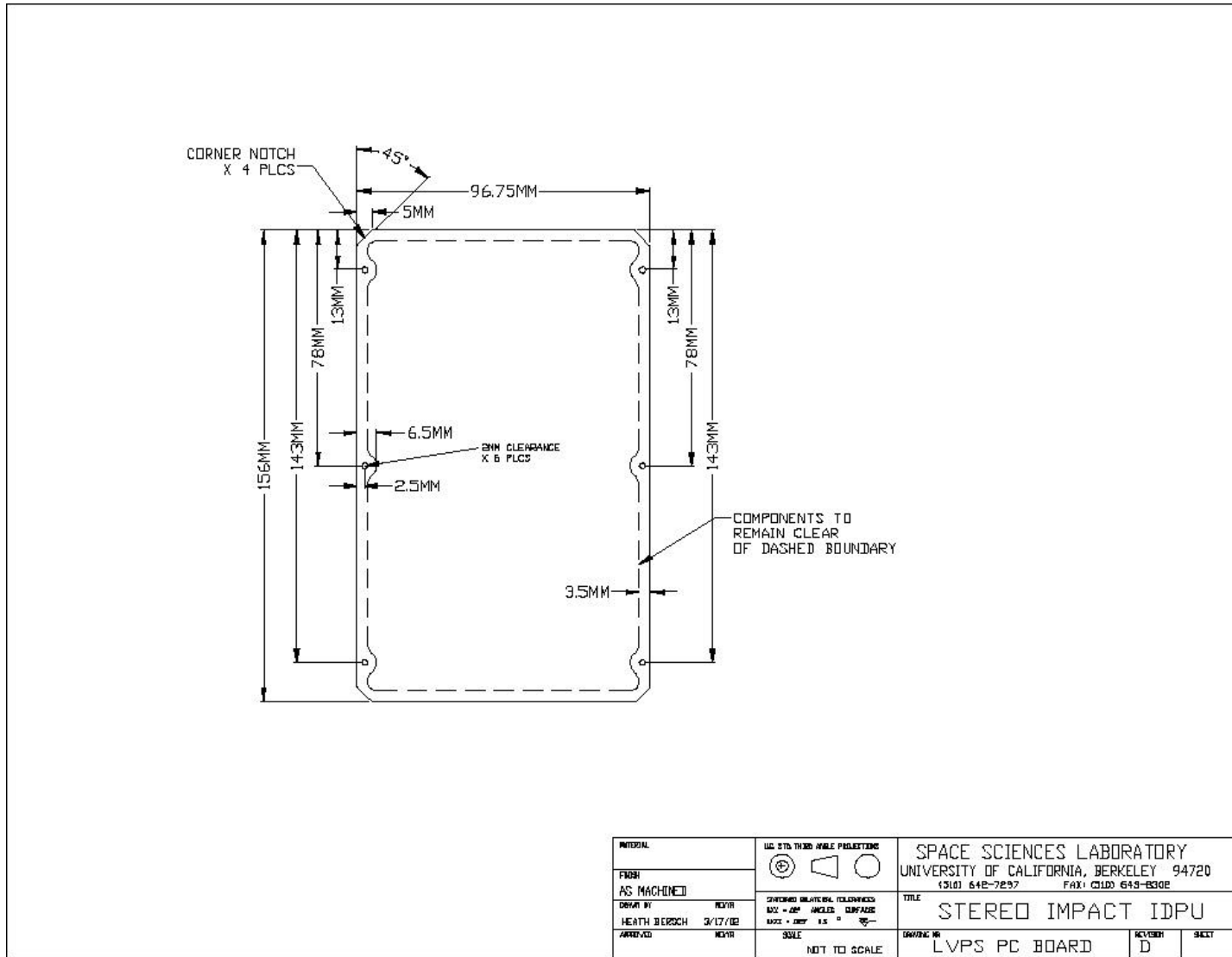
Figure 6 – LVPS Board Outline
