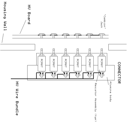
HU CONNECTOR ASSEMBLY
