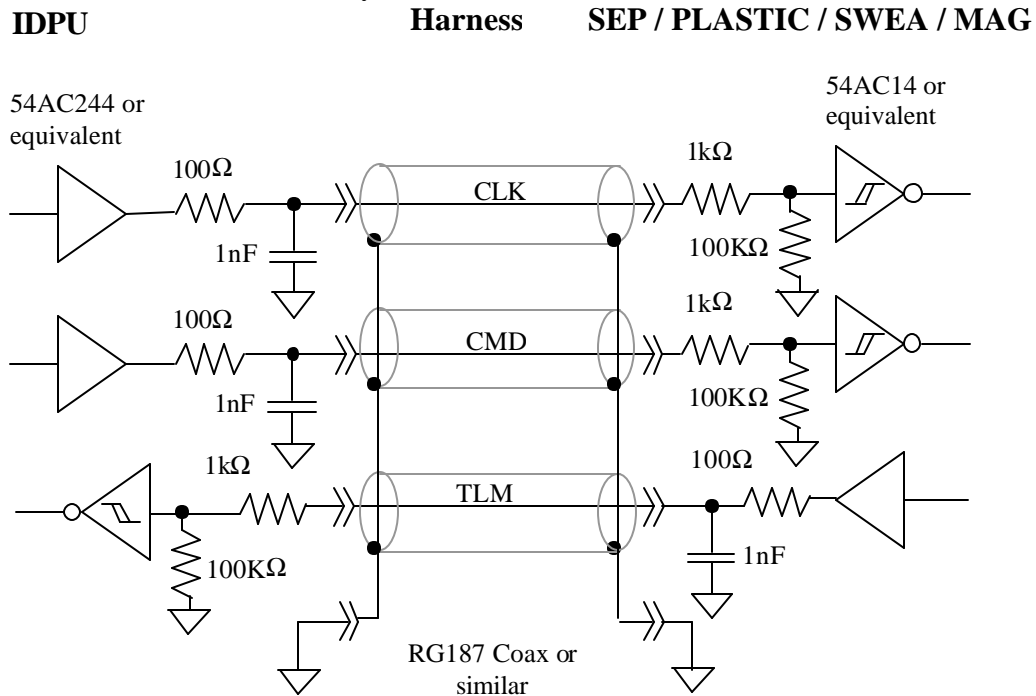
Figure 1 - Serial Interface Circuit
