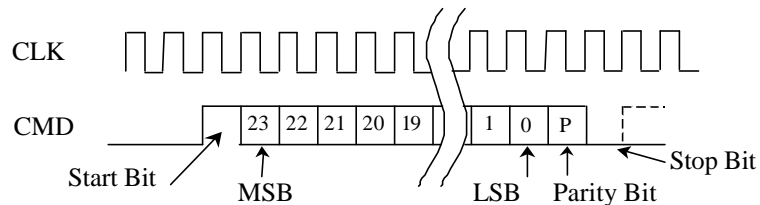
Figure 2 - Serial Command Timing
