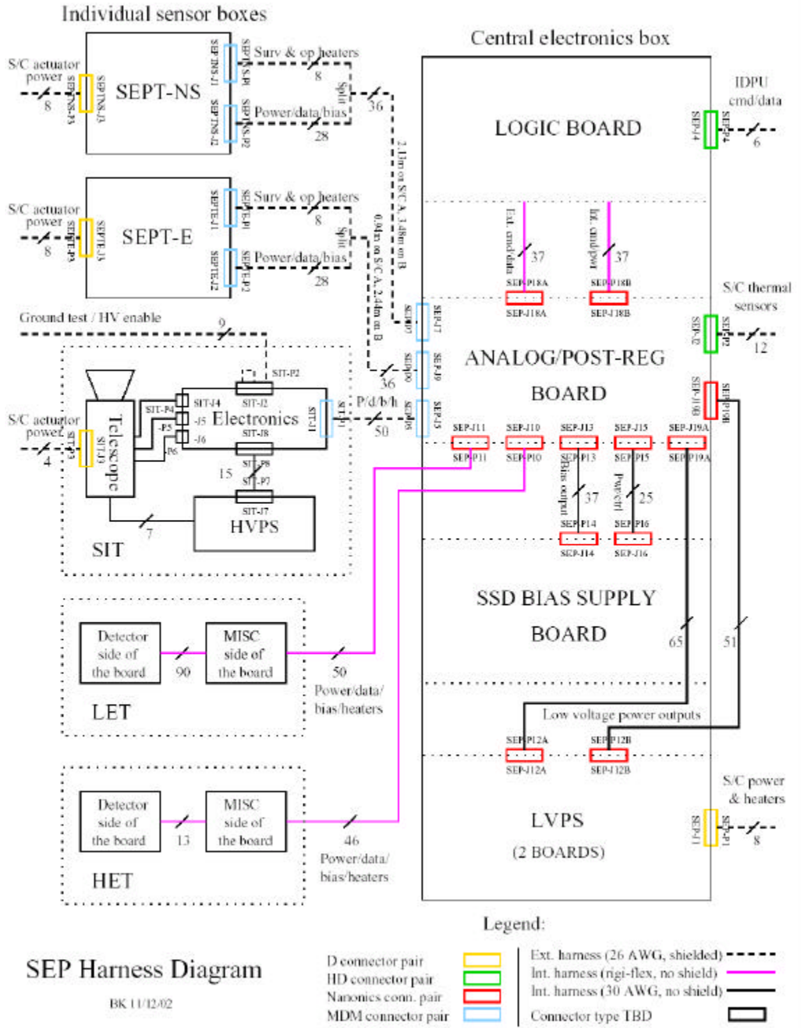
Figure 2-2 SEP Harness
