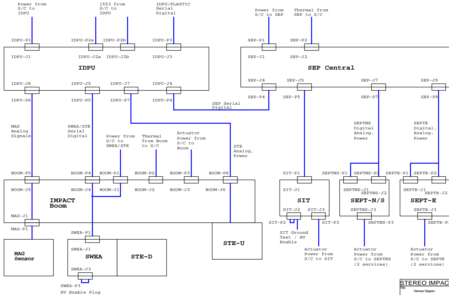
Figure 2-1 - IMPACT Harness Schematic
