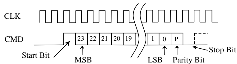
Figure 2 - Serial Command Timing
